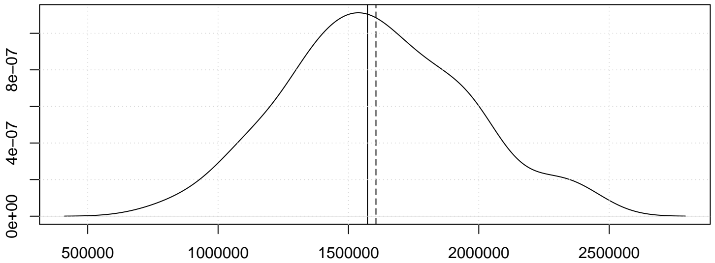
Density Plot – Gaussian Kernel
