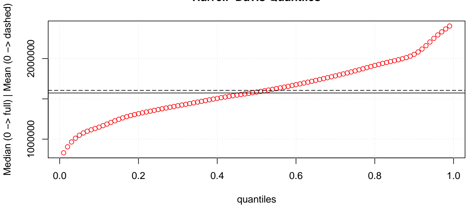
Harrell-Davis Quantiles
