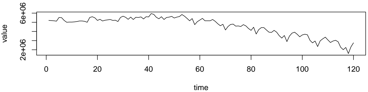
Working Time Series (lambda=1, d=0, D=0)
