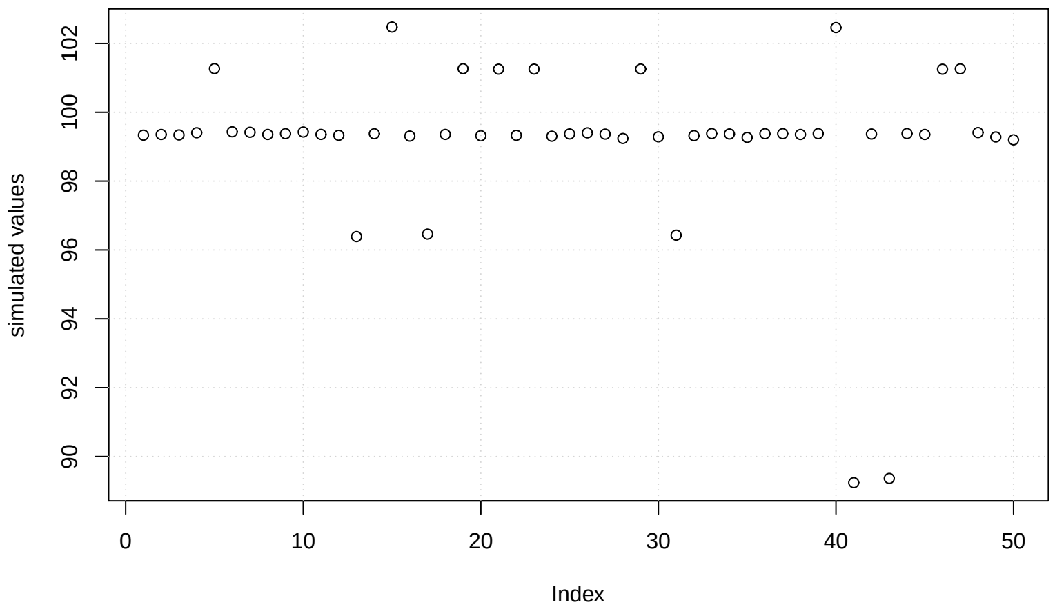
Simulation of Mode of Kernel Density
