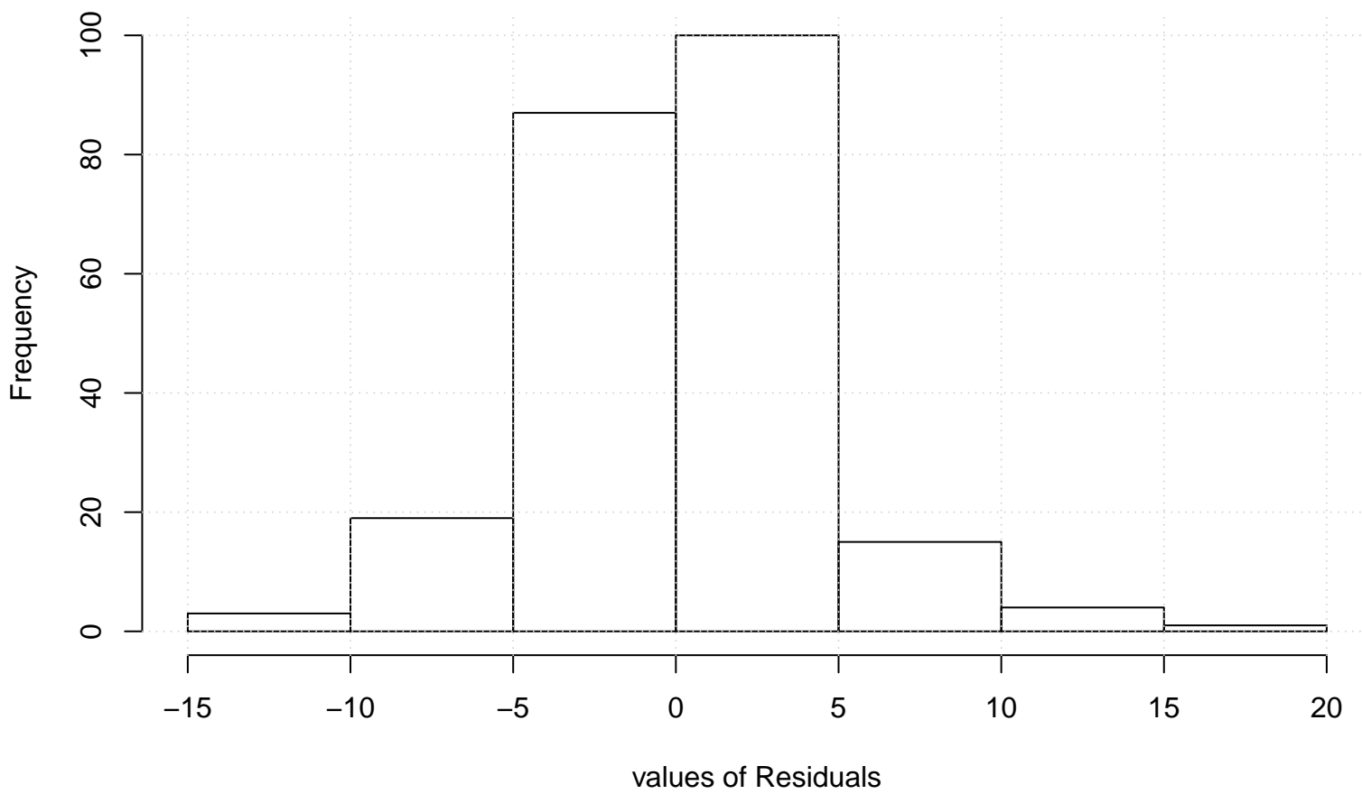
Residual Histogram
