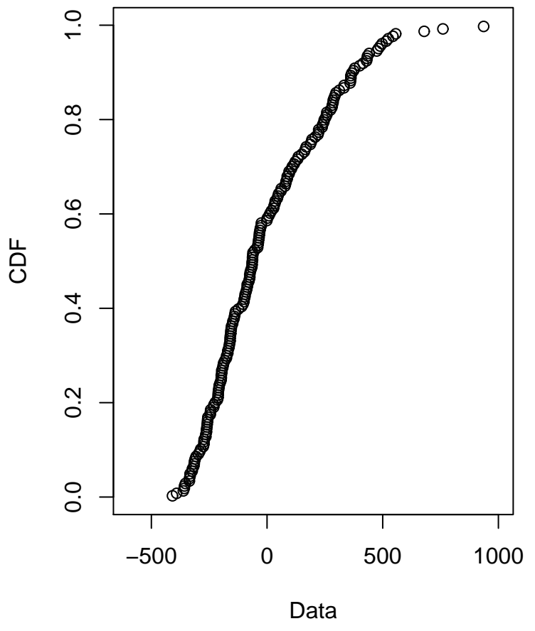
Cumulative distribution
