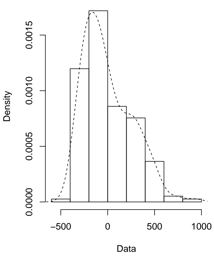
Empirical density
