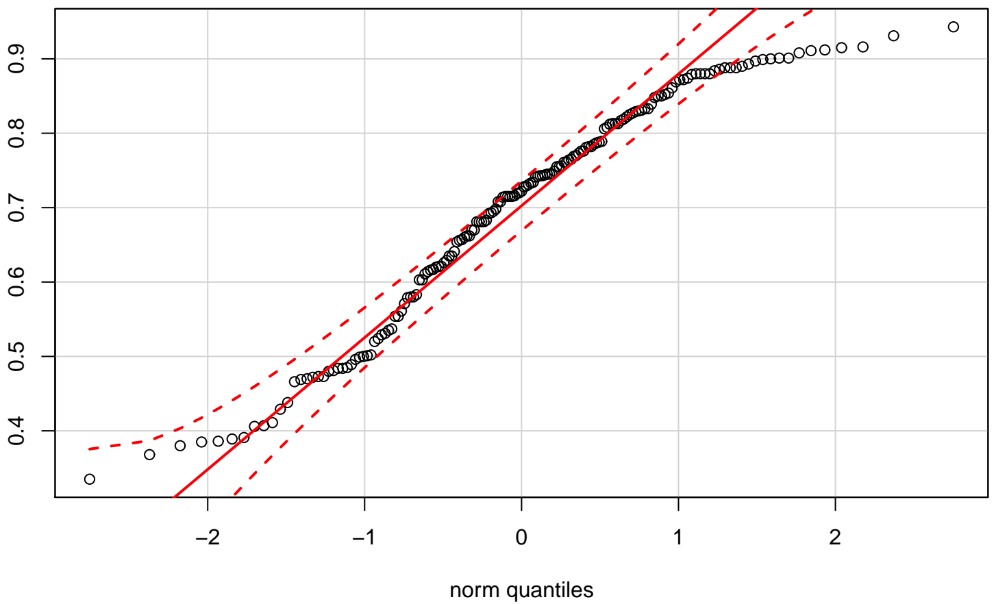
QQplot of variable x
