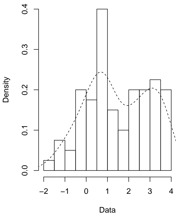
Empirical density
