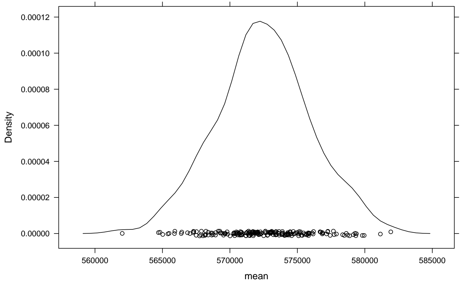
Density Plot
