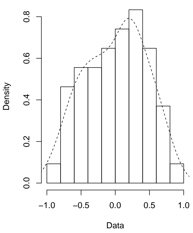
Empirical density
