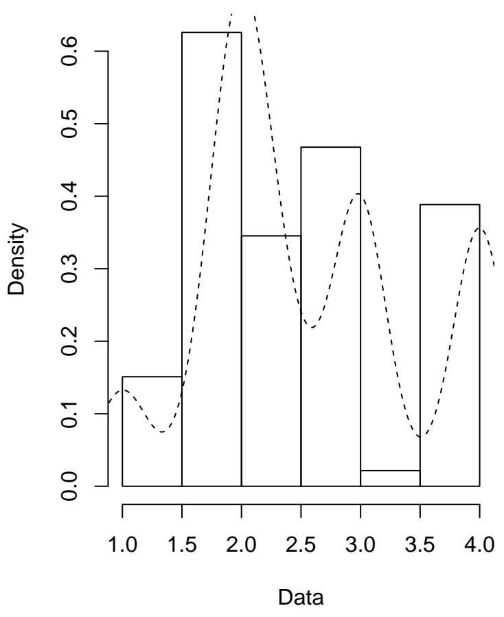
Empirical density
