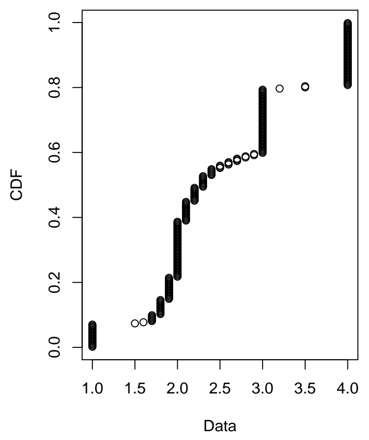
Cumulative distribution
