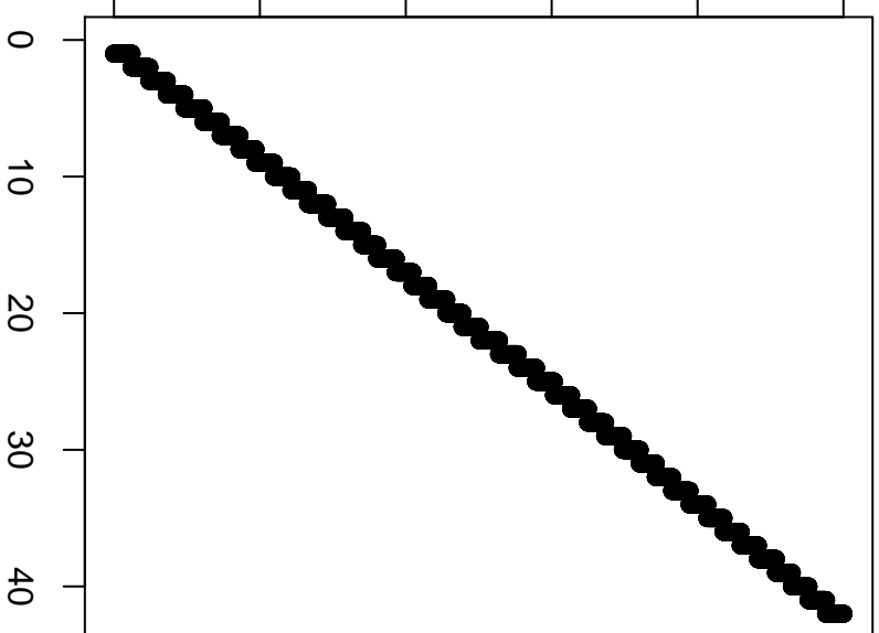
Cumulative distribution
