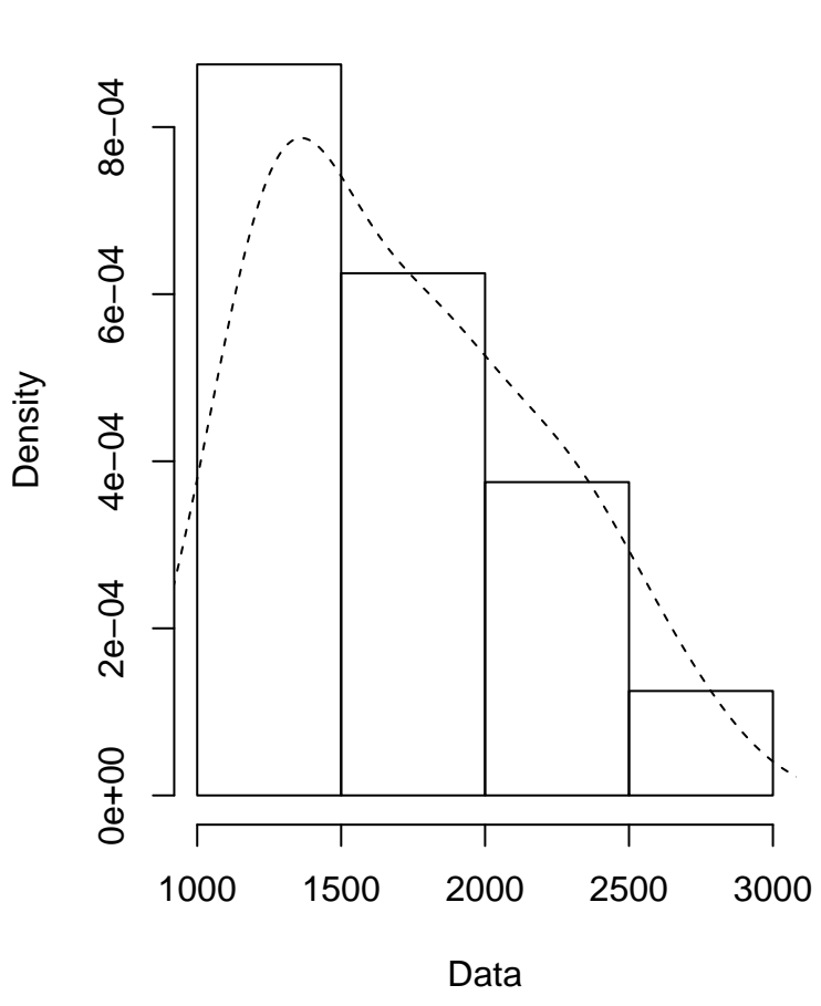
Empirical density
