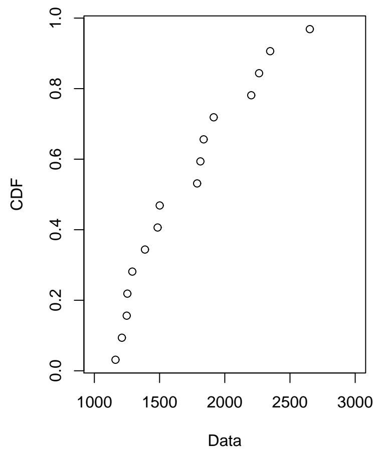
Cumulative distribution
