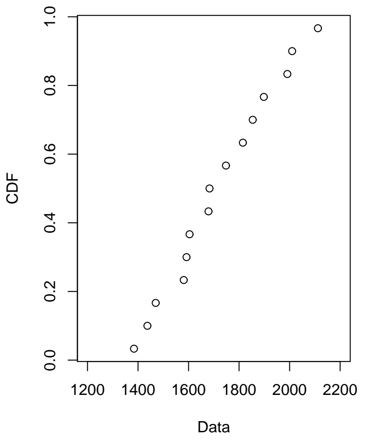
Cumulative distribution
