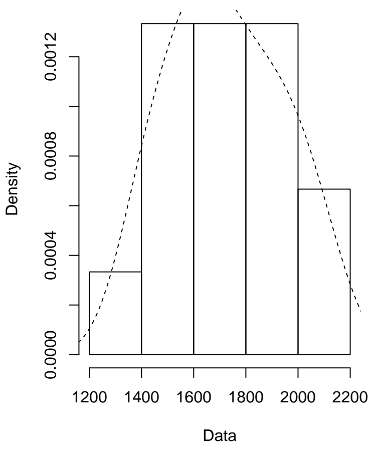
Empirical density
