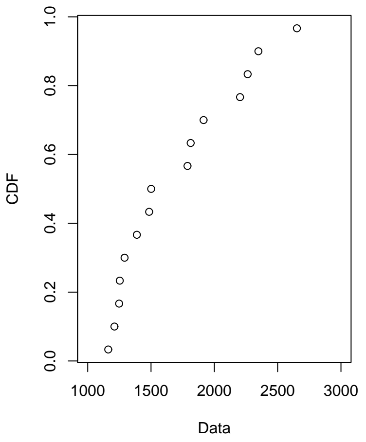
Cumulative distribution
