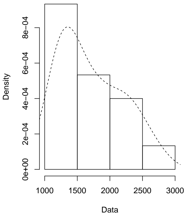
Empirical density
