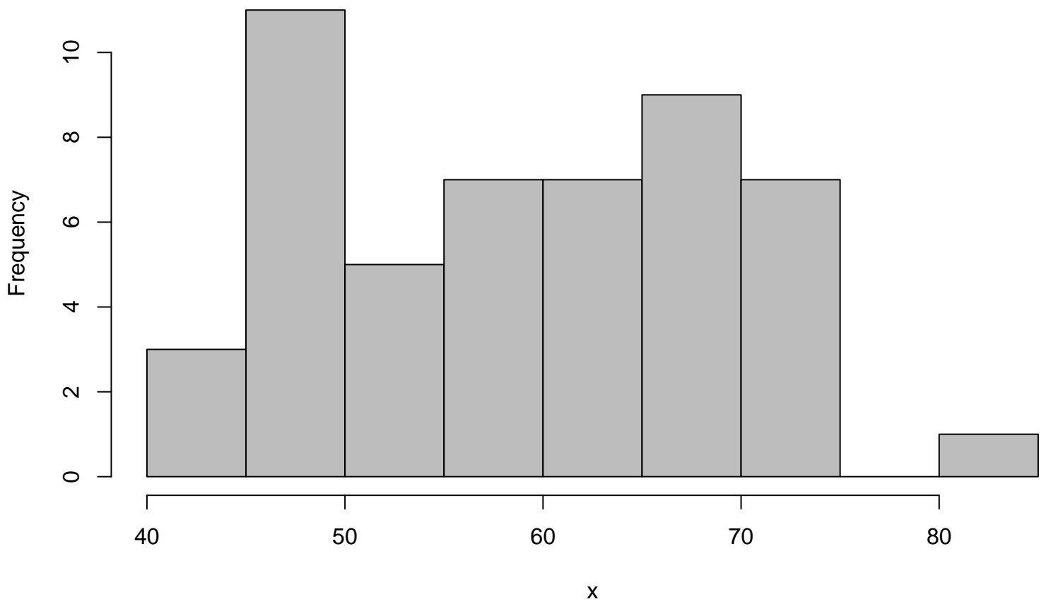
Histogram
