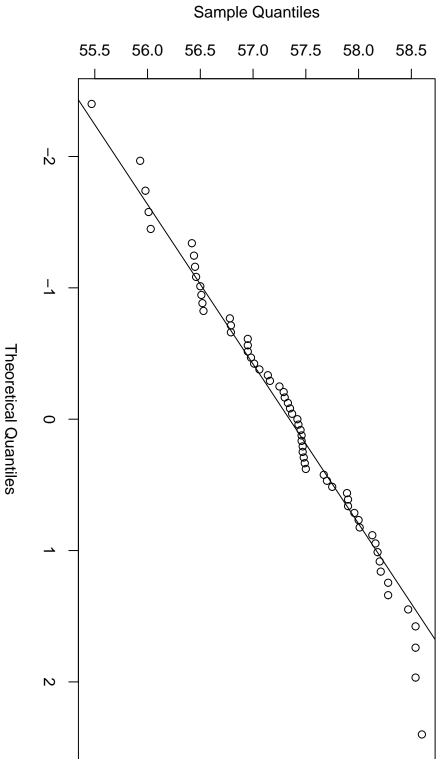
Normal Q-Qplot – Variable 2
