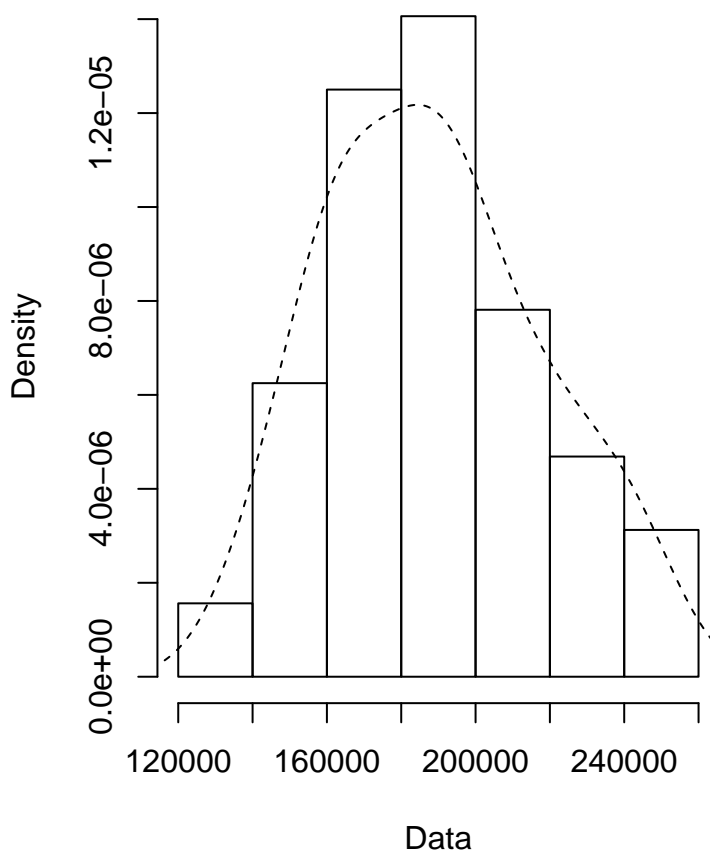
Empirical density
