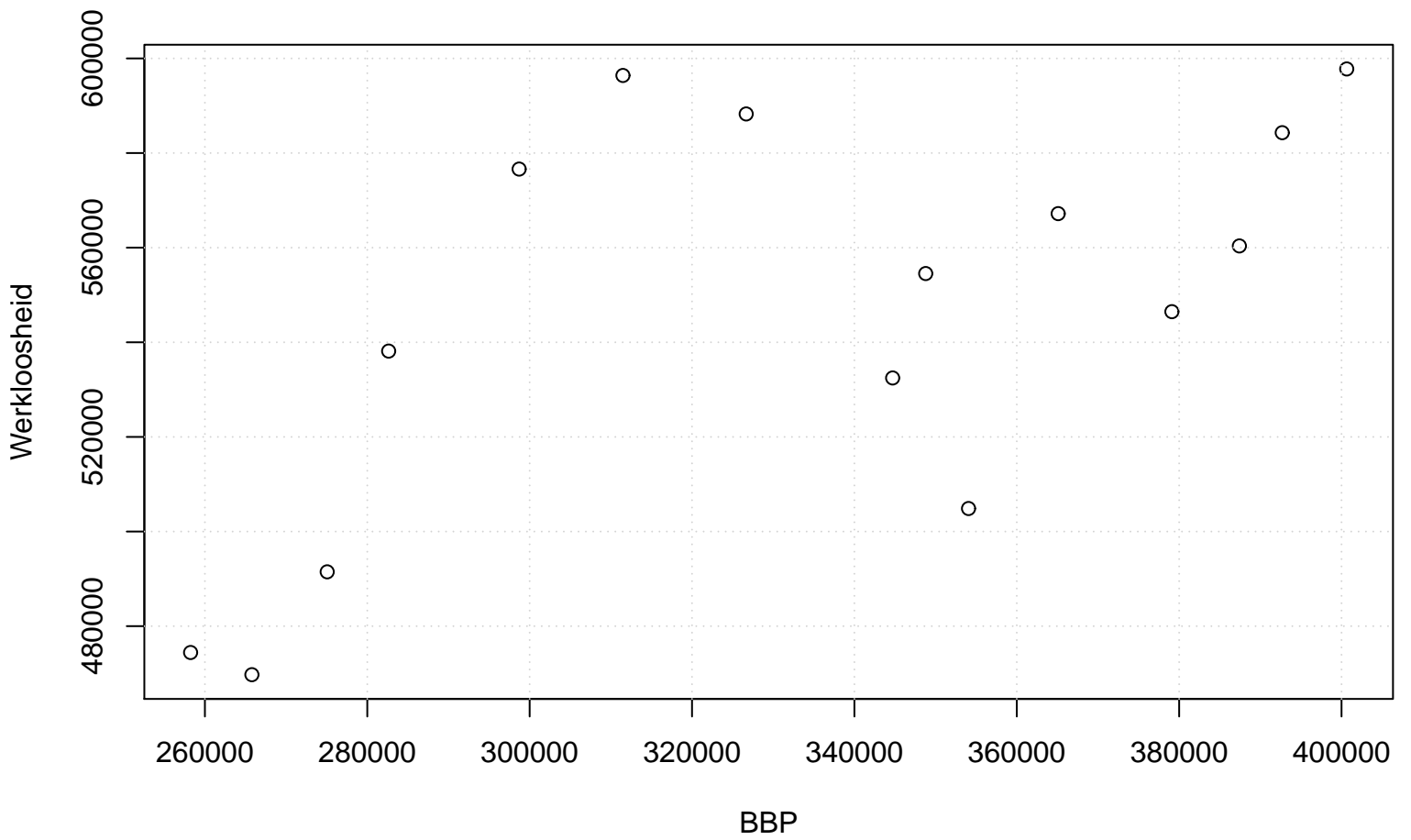
Scatterplot
