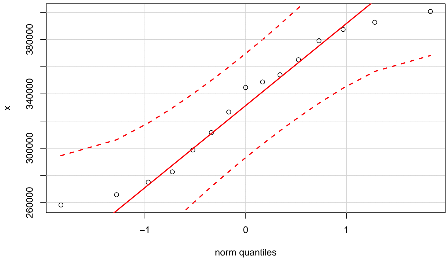
QQ plot (Normal) with confidence intervals
