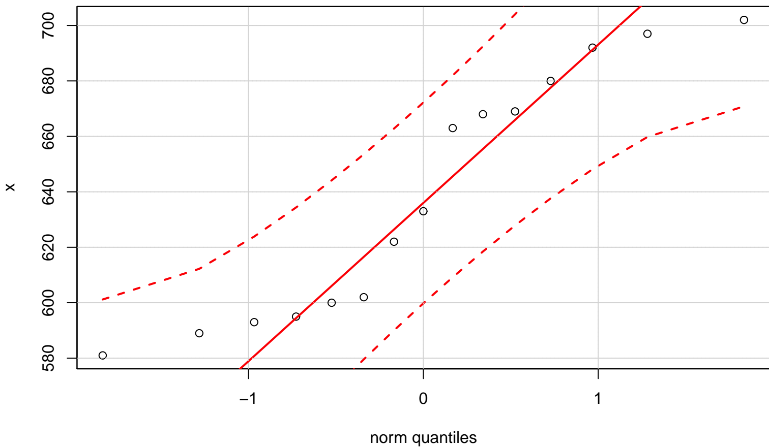
QQ plot (Normal) with confidence intervals
