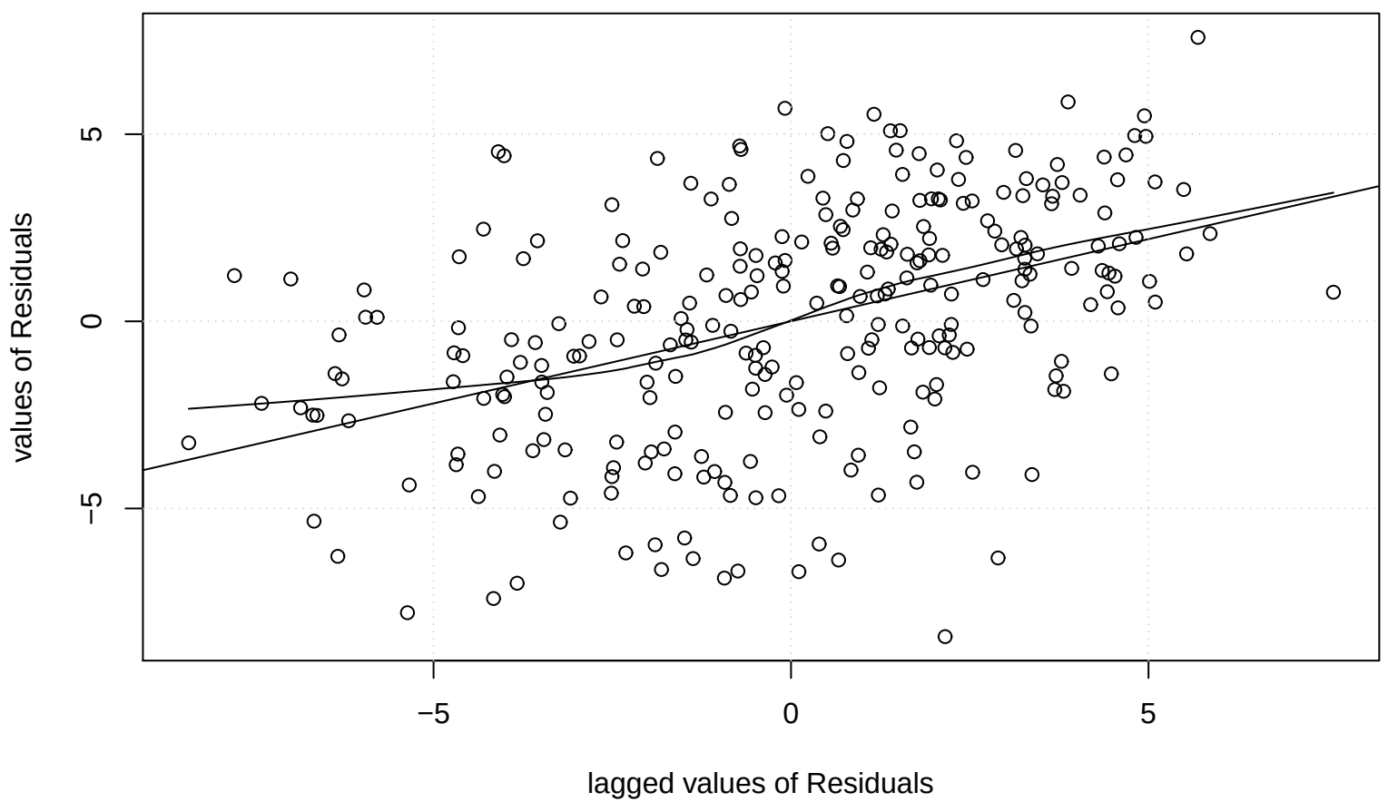
Residual Lag plot, lowess, and regression line
