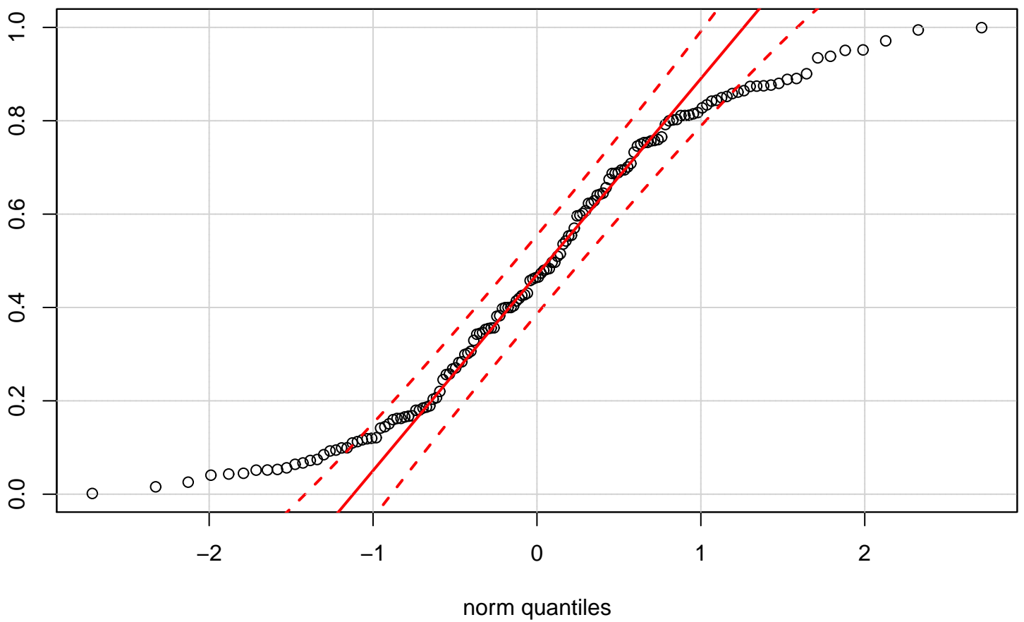
QQ plot (Normal) with confidence intervals
