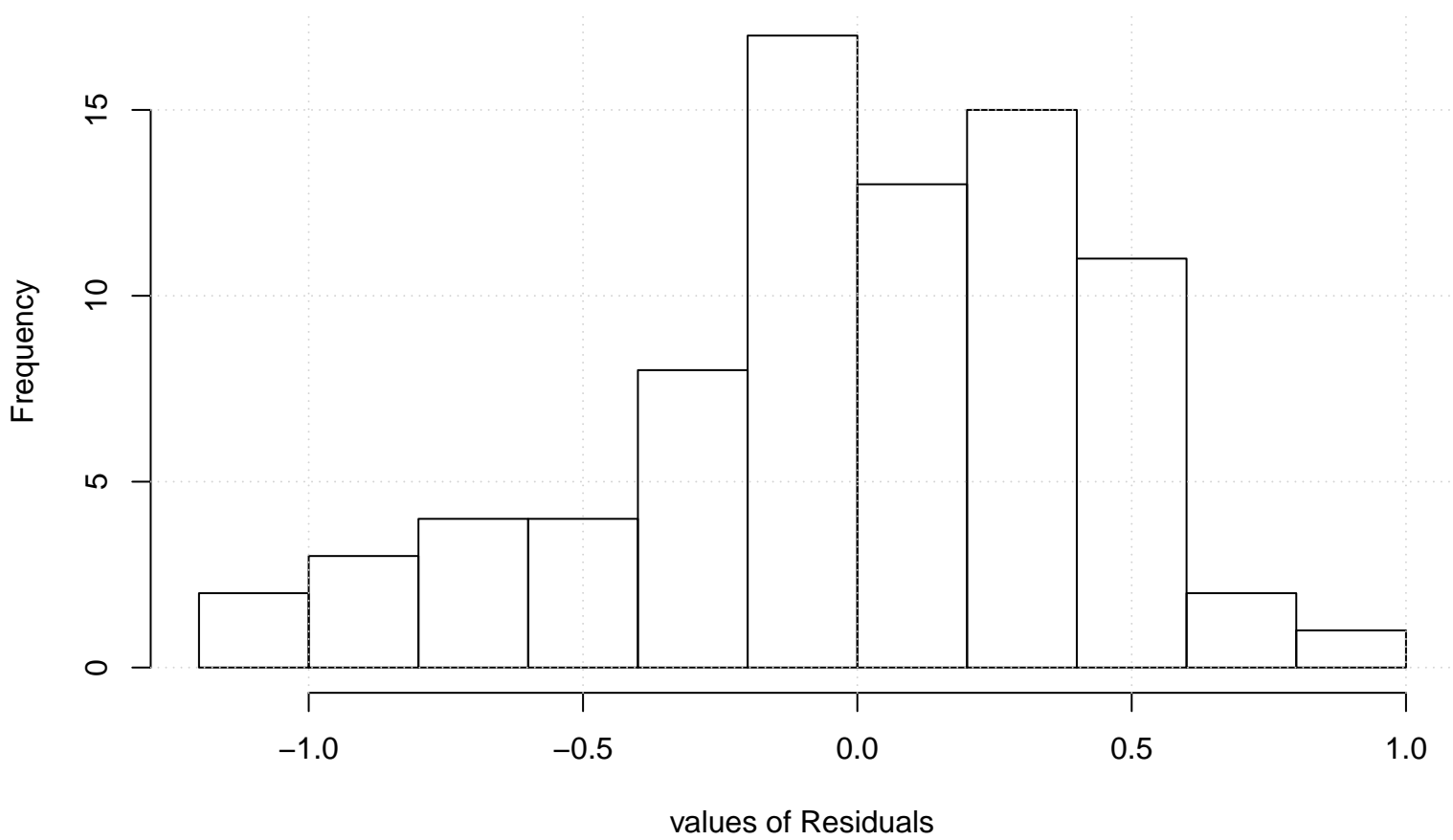
Residual Histogram
