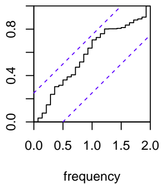
Residual Cumulative Periodogram
