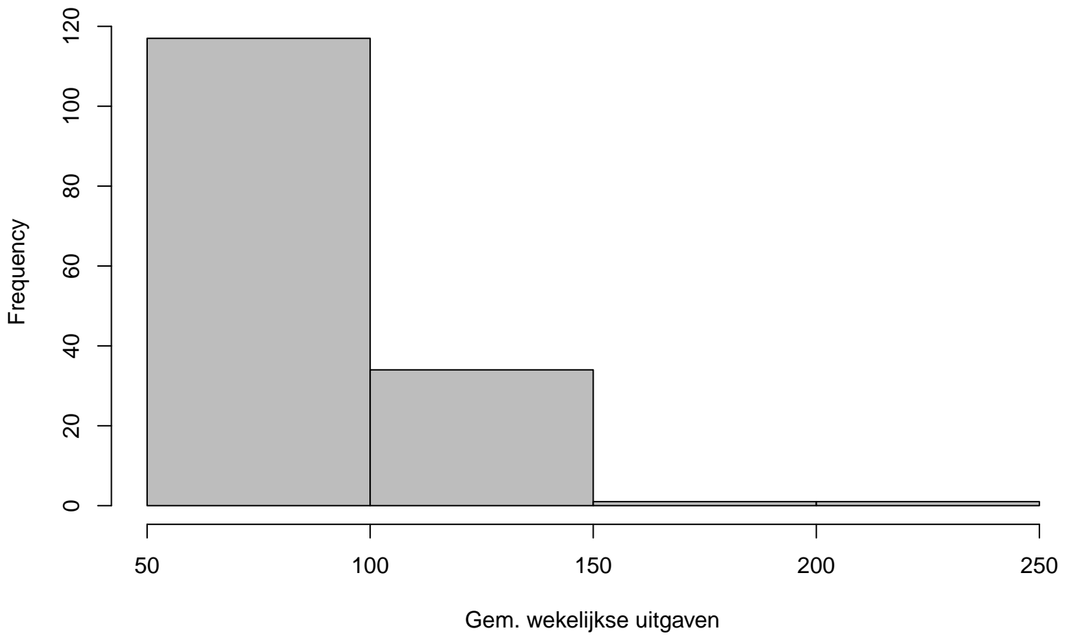
Histogram supermarkt
