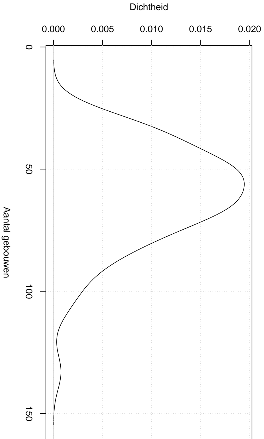
Gaussian Kernel
