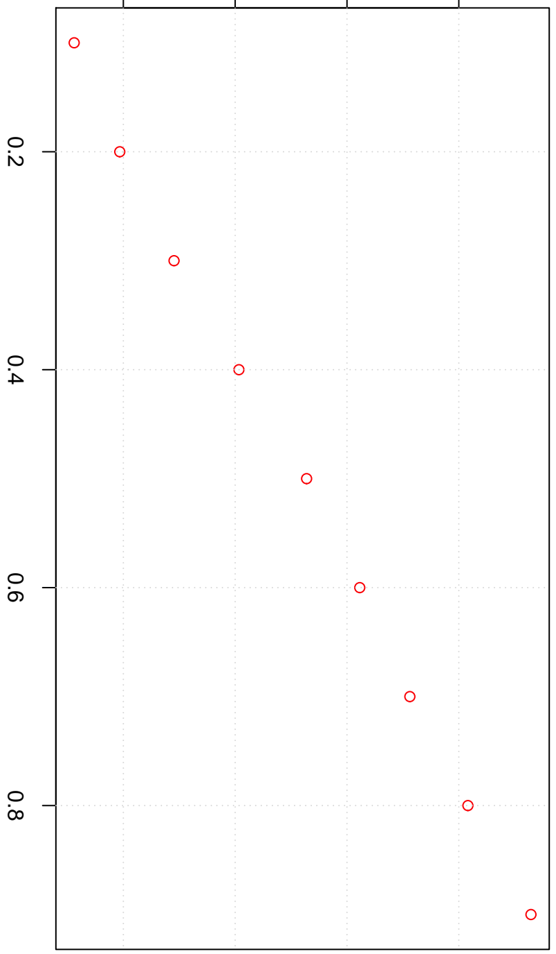
Harrell-Davis Quantiles
