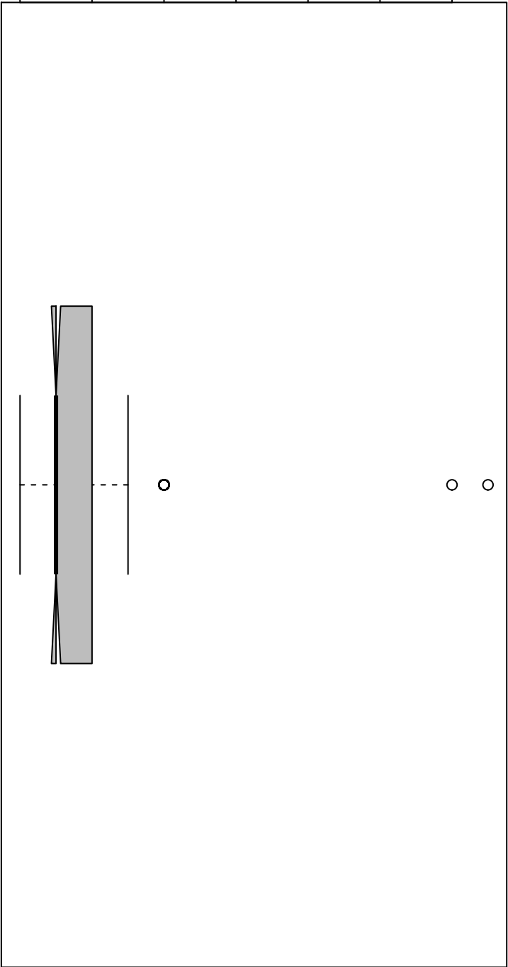
Notched Boxplots
