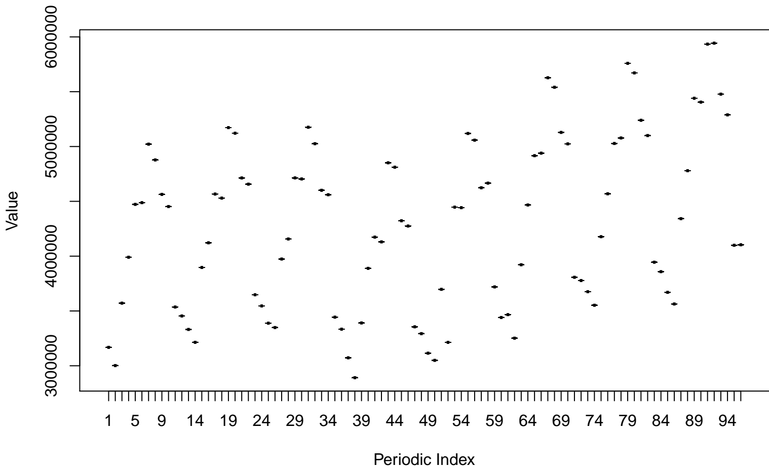
Notched Box Plots – Periodic Subseries
