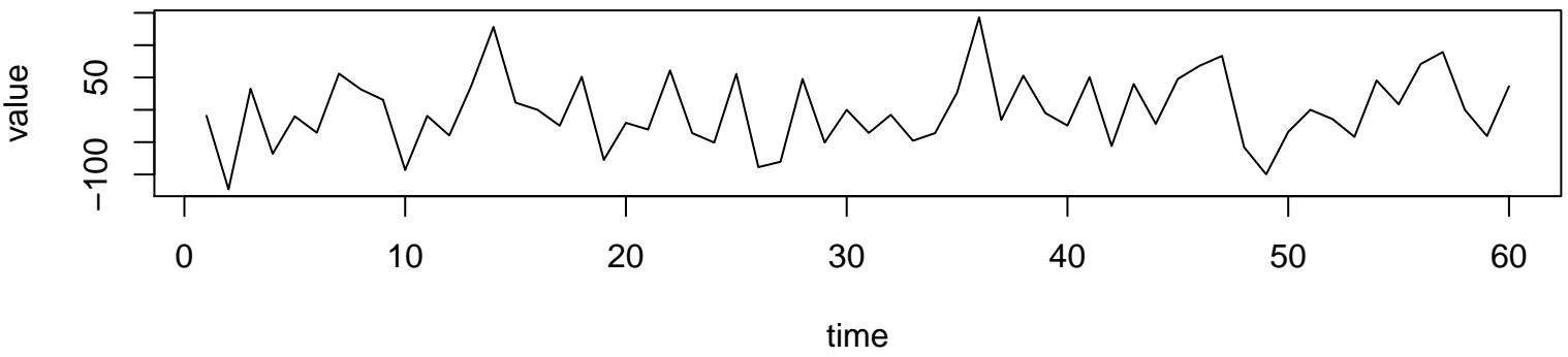
Working Time Series ( \lambda=1.4 , d=0 , D=1 )
