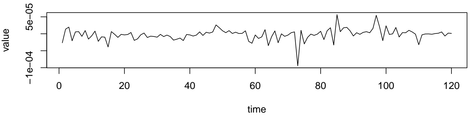
Working Time Series ( \lambda=-1.1 , d=0 , D=1 )
