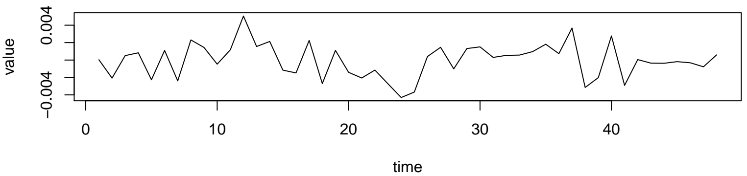
Working Time Series ( \lambda=-0.3 , d=0 , D=2 )
