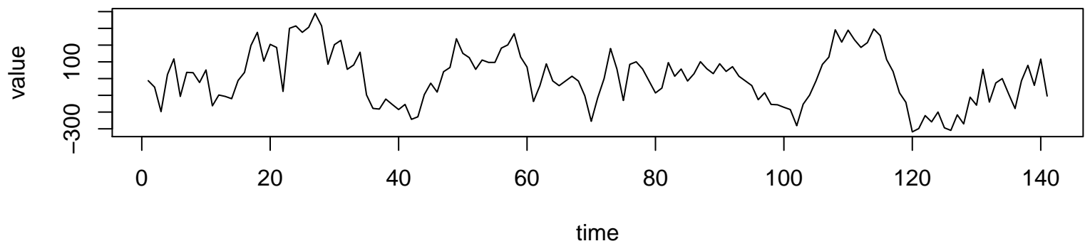
Working Time Series ( \lambda=1.6 , d=0 , D=1 )
