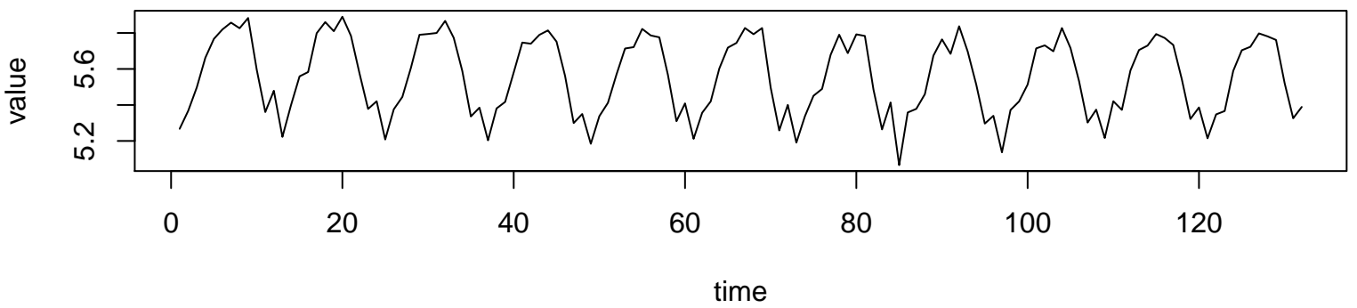
Working Time Series ( \lambda=-0.1 , d=0 , D=0 )
