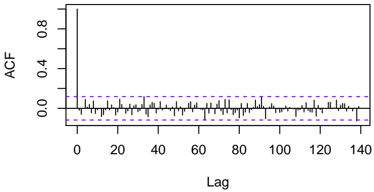
Residual ACF
