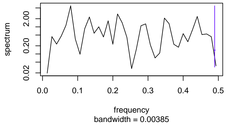
Standardized Residuals
