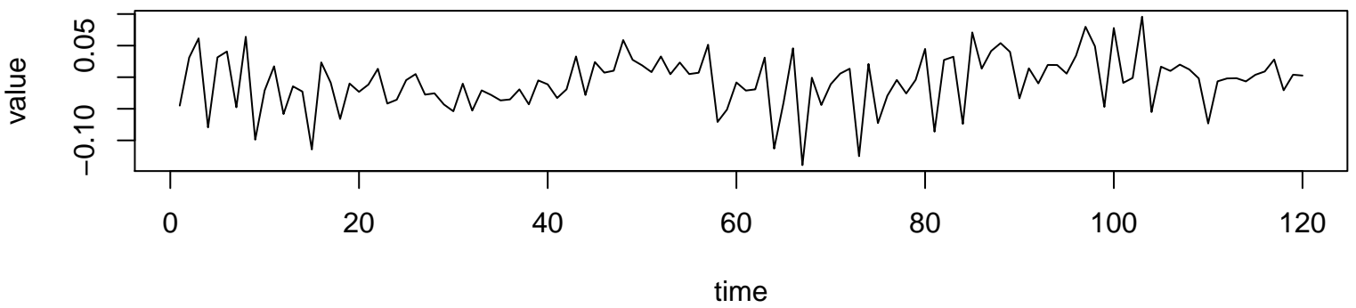
Working Time Series ( \lambda=-0.1 , d=0 , D=1 )
