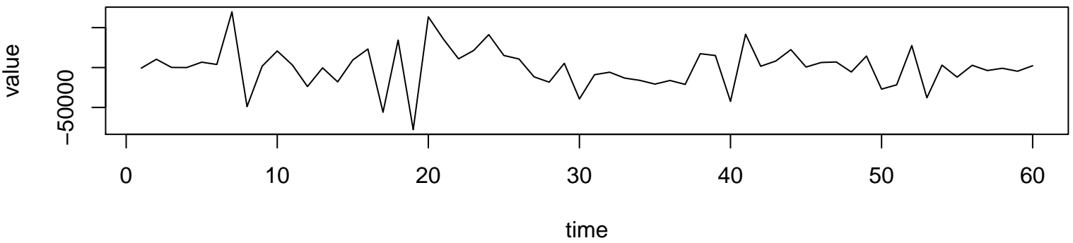
Working Time Series (lambda=0.9, d=0, D=1)
