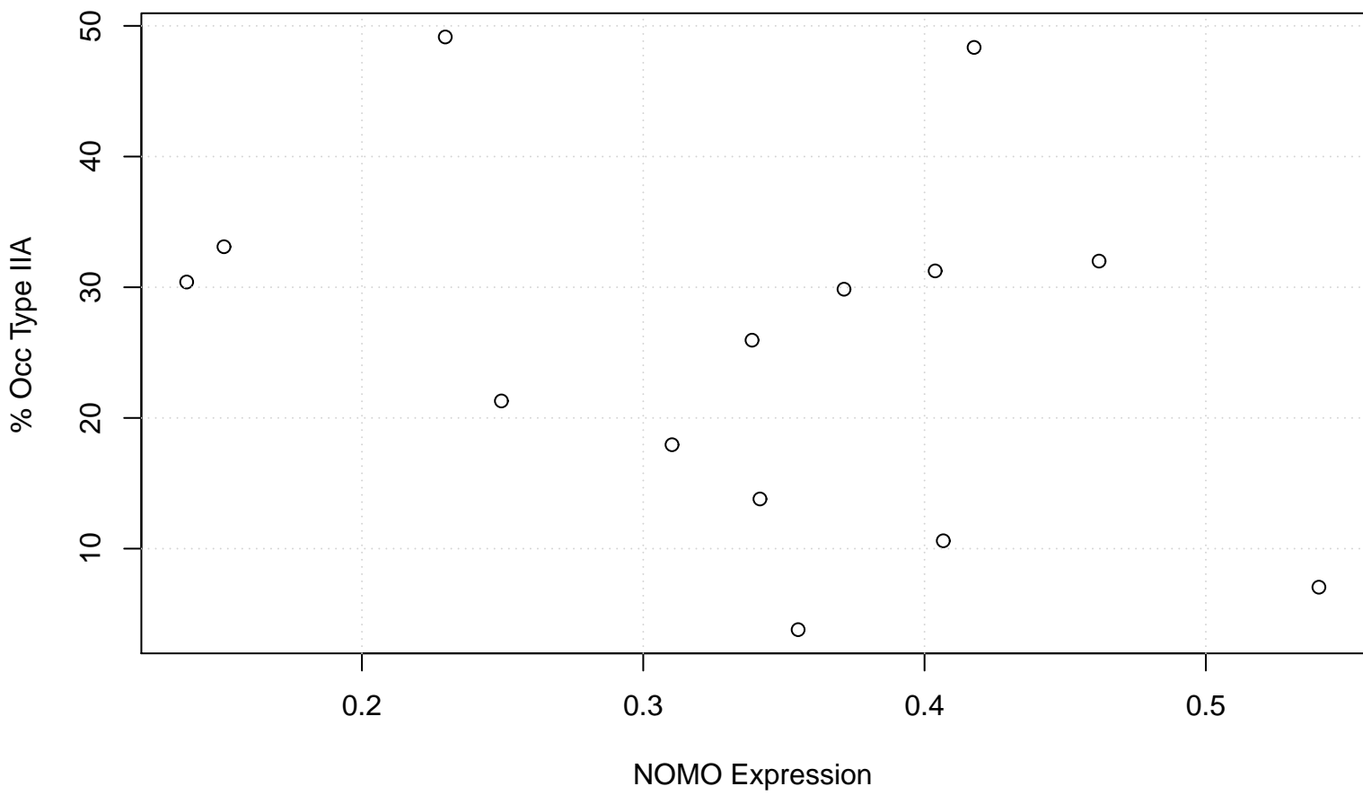
Scatterplot
