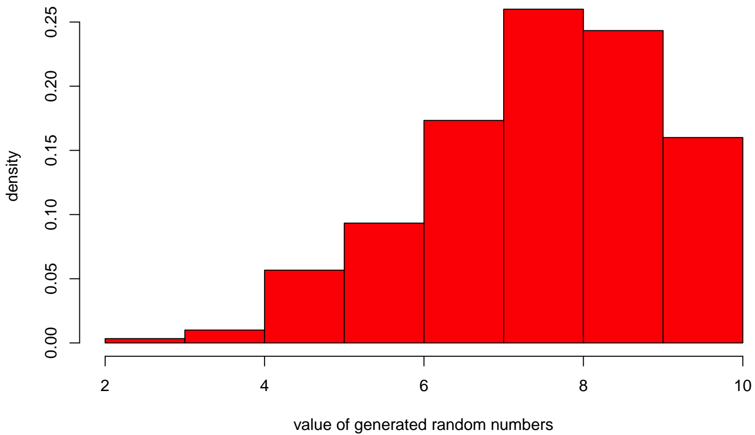
Histogram of Generated Random Numbers
