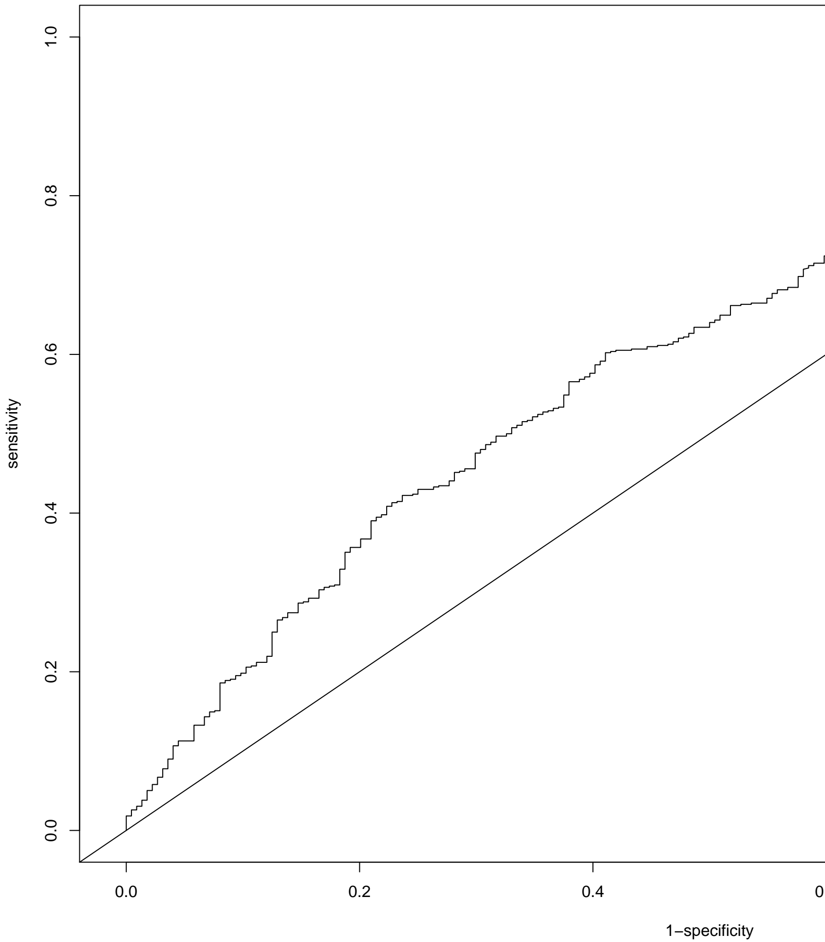
ROC plot
