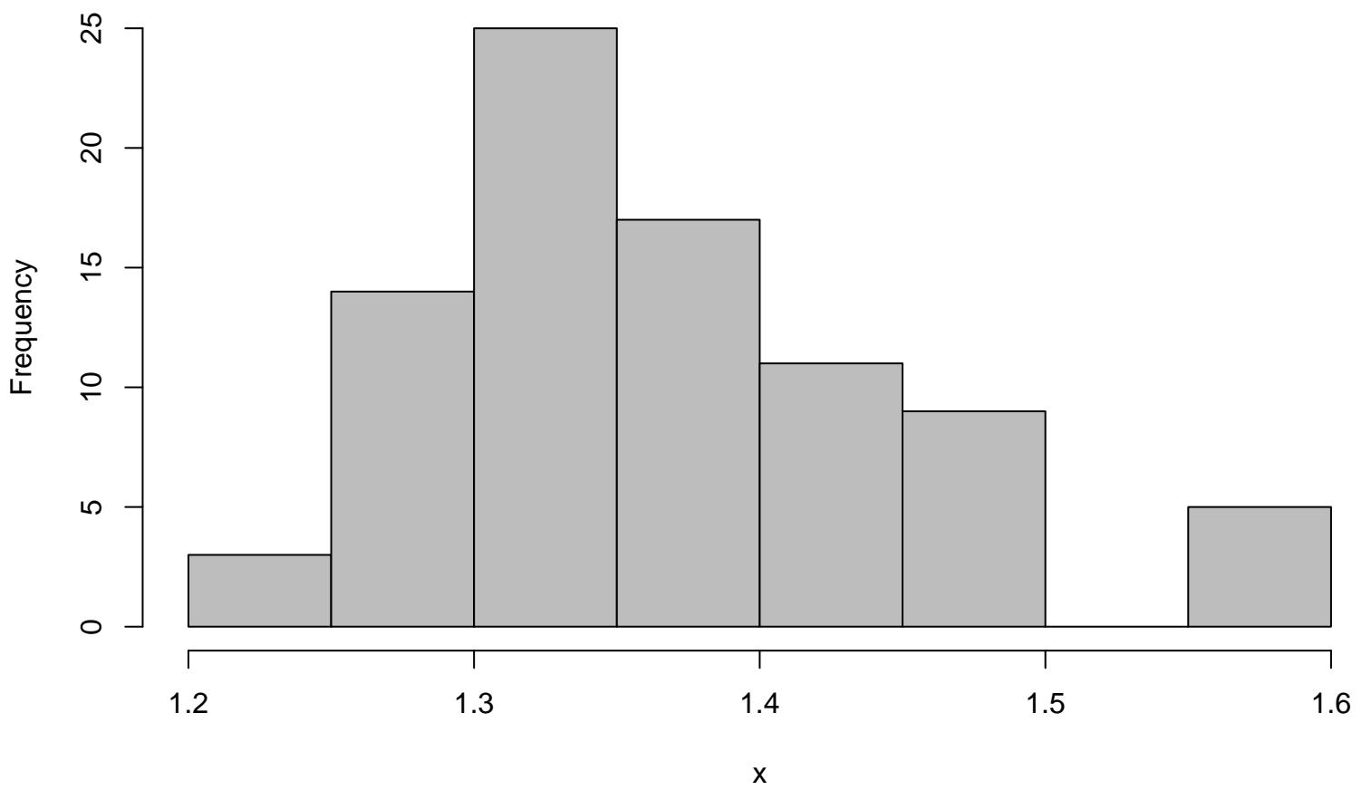
Histogram
