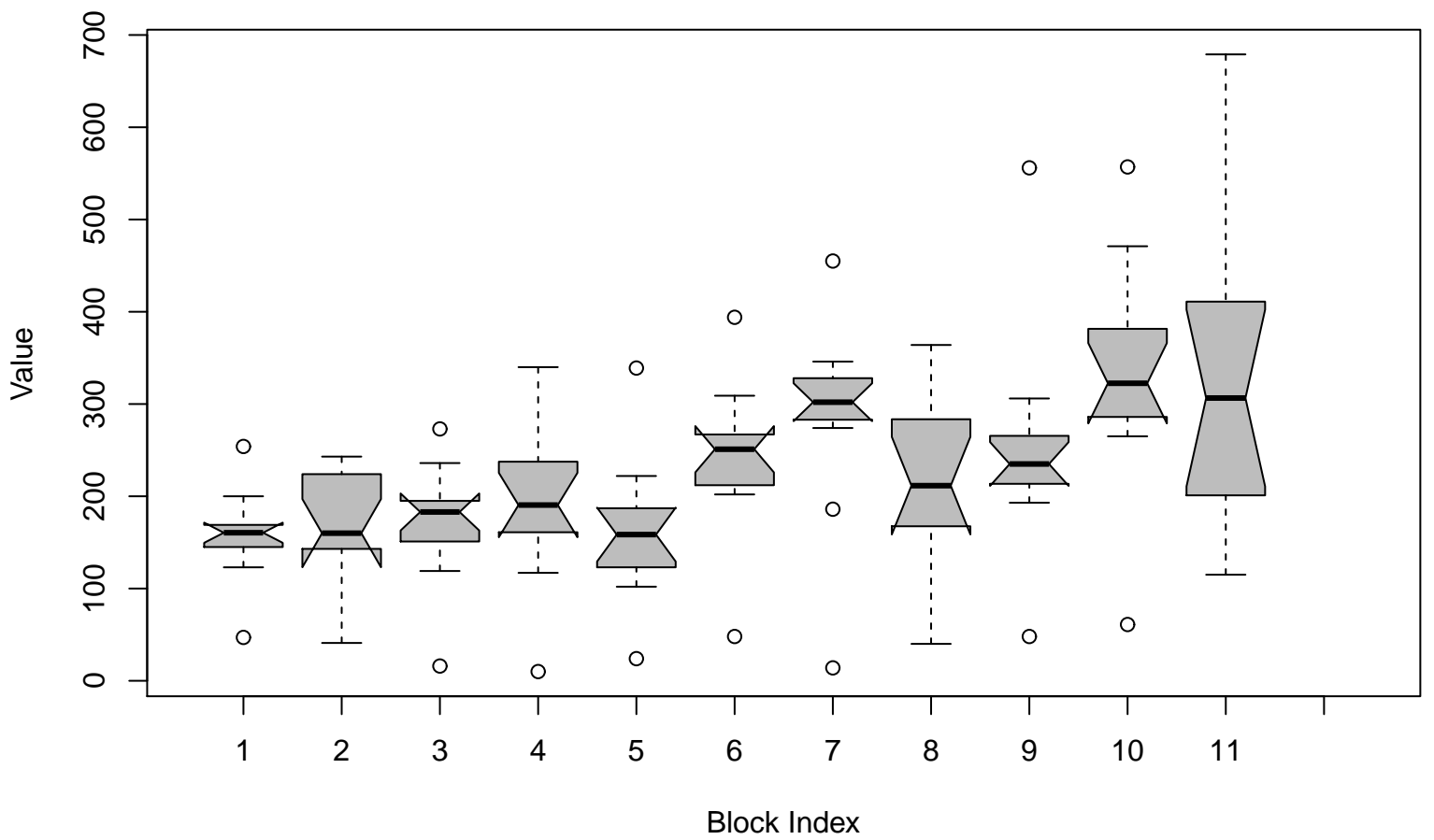
Notched Box Plots – Sequential Blocks
