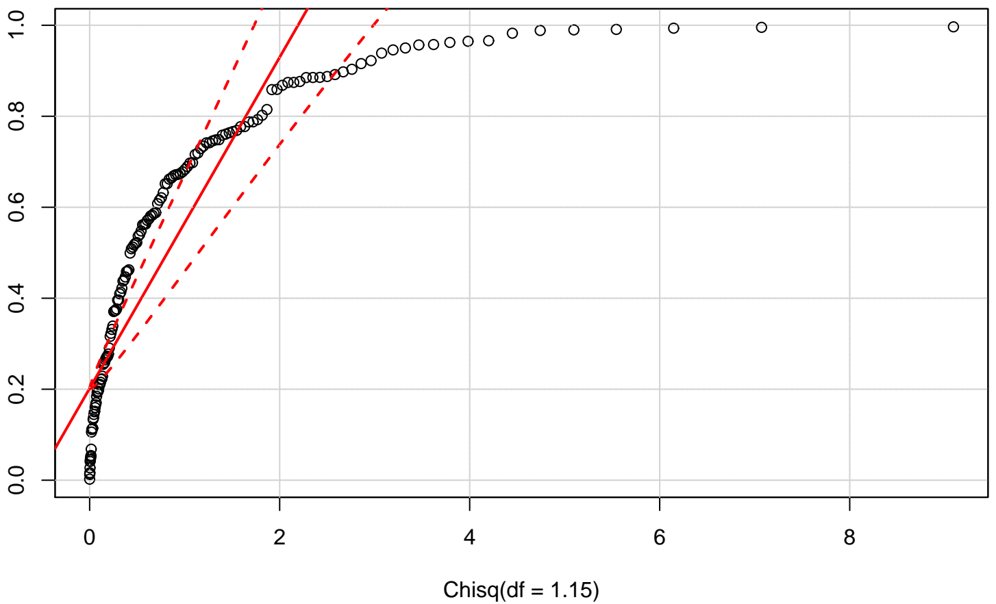
QQ plot (Chi-squared 1 param.)
