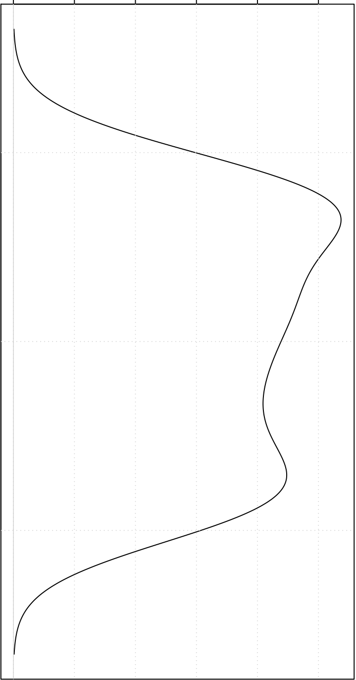
Gaussian Kernel
