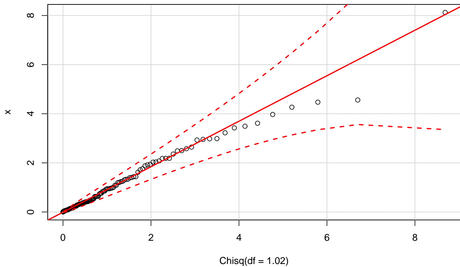
QQ plot (Chi-squared 1 param.)
