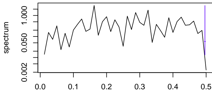
frequency bandwidth = 0.00361
