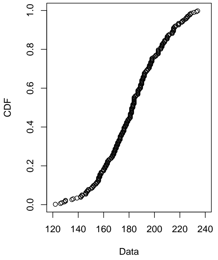
Cumulative distribution
