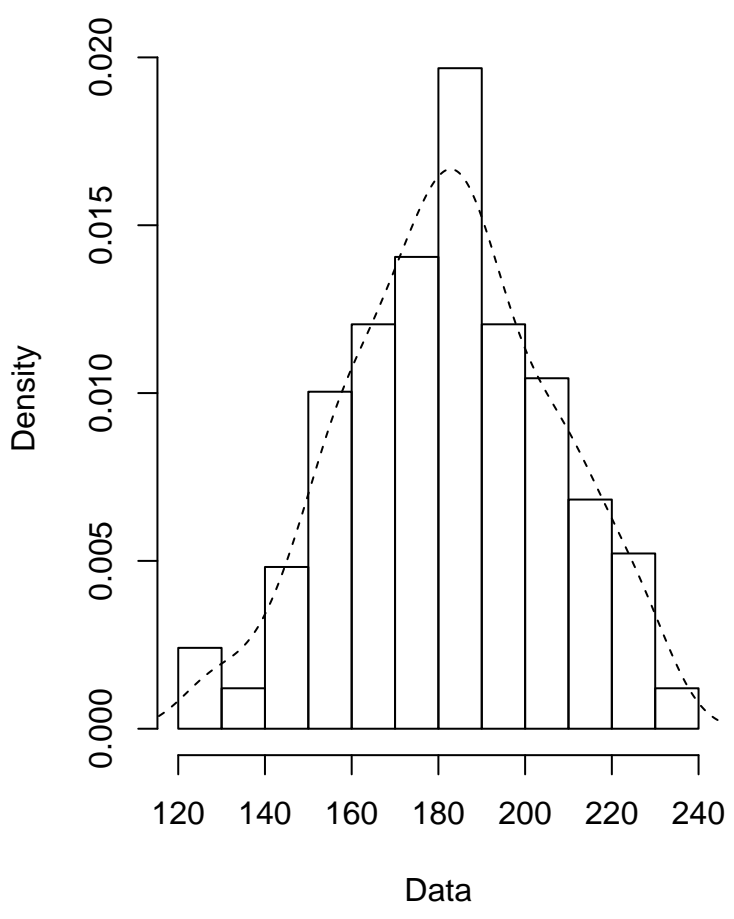
Empirical density
