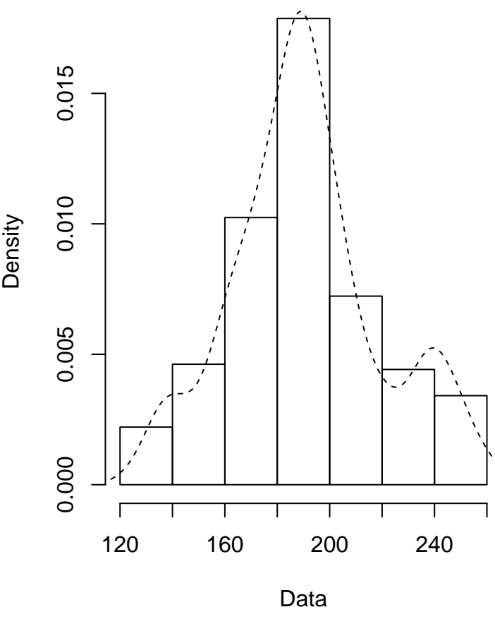
Empirical density
