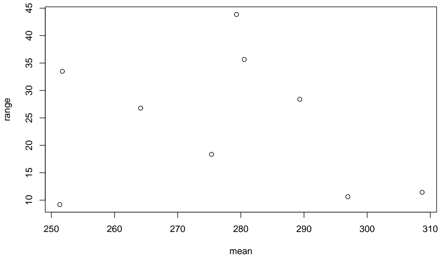
Range–Mean Plot
